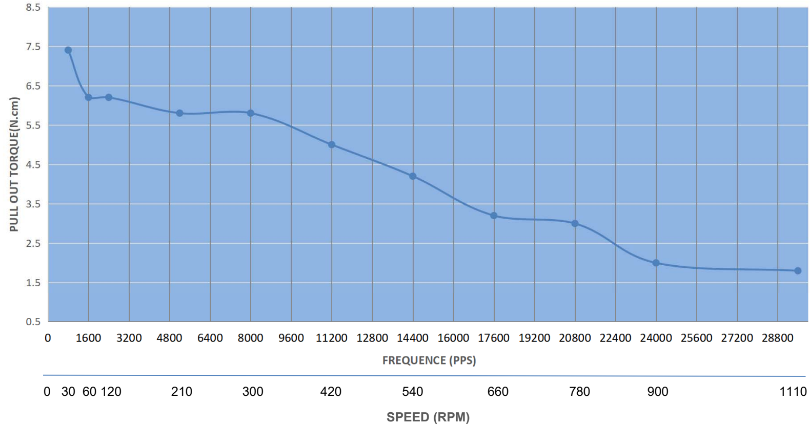
PULL OUT TORQUE CURVE OF 14HS08-0404S
