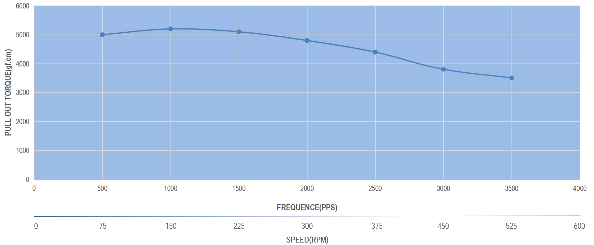
17HS24-2104D-E1000 PULL OUT TORQUE (2.1A/PHASE 24V CONSTANT CURRENT HALF STEP)
