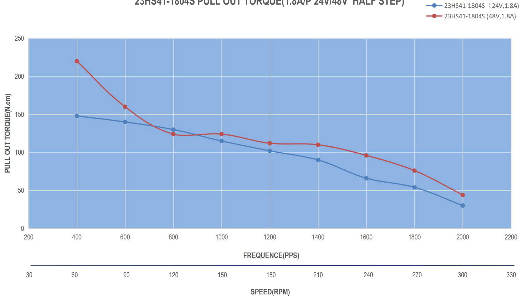
23HS41-1804S PULL OUT TORQUE(1.8A/P 24V/48V HALF STEP)
