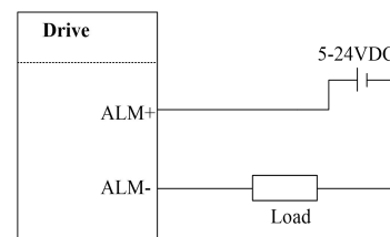
Figure 7 Sourcing output
