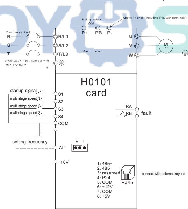
wiring diagram of carving maching inverter
