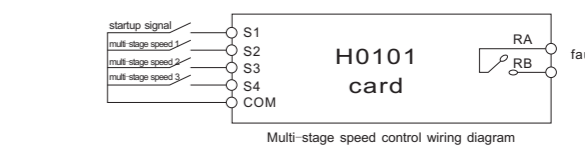
Multi-stage speed control wiring diagram
