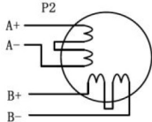
Figure 7: 8-lead motor series connections
