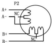
Figure 6: 6-lead motor full coil (higher torque) connections
