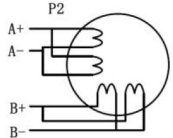
Figure 9: 8-lead motor parallel connections
