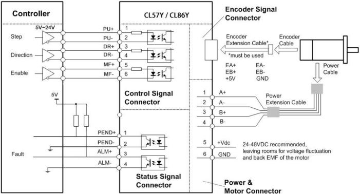
Figure 3: Typical connection
