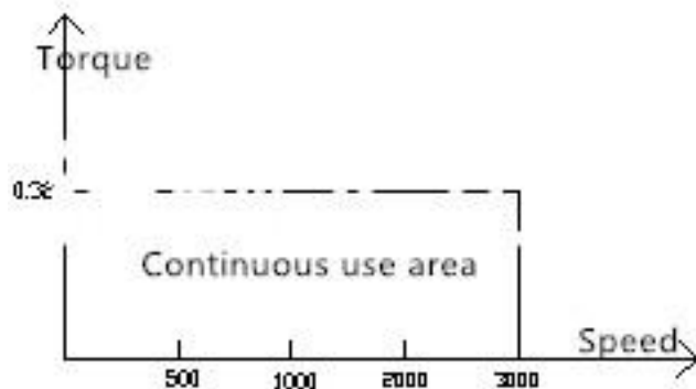
iHSV57-30-10-36-XXX4/5000 Torque characteristics
